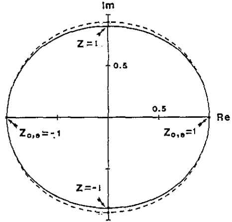
Figure 4. Quartic loci of t_o (solid curve) and t_e (dashed curve). The t_o -quartic is fixed, while the t_e -quartic depends on the direction cosine \gamma of the optic axis relative to the surface normal. The curves are drawn for calcite in air, as in figure 1, with \gamma = 0 (optic axis in the reflecting plane). The values of Z = \exp(ik \Delta z) are shown at special points.
