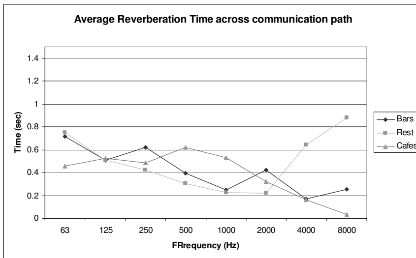
Figure 2: Third Octave Band Reverberation Times.
