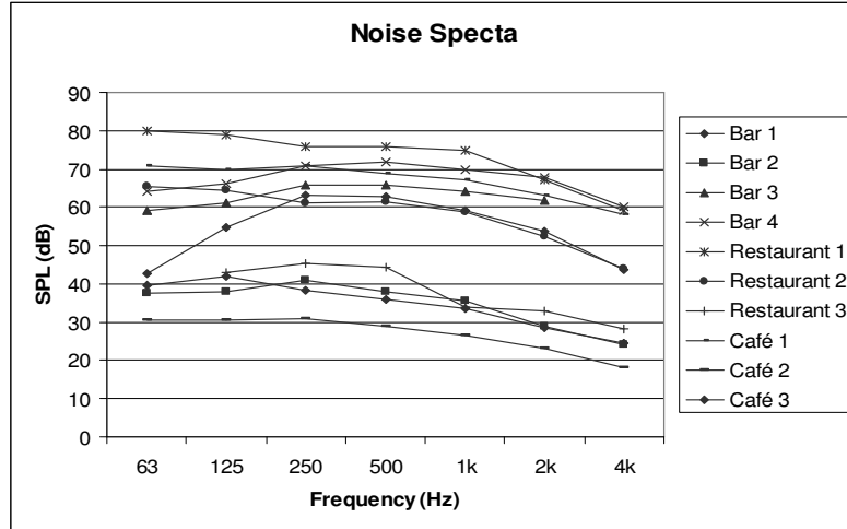
Figure 1: Noise Spectra of each Venue.
