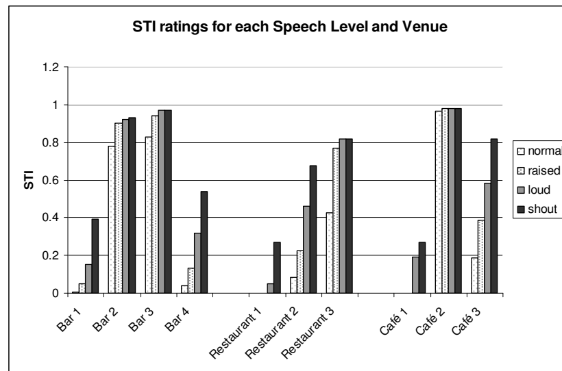
Figure 3: STI Ratings for each Speech Level and Venue.
