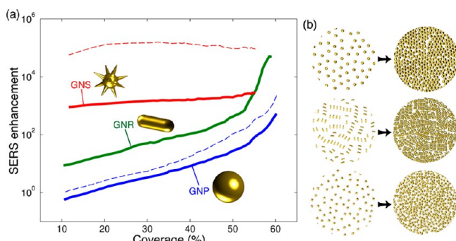
Figure 2. Predicted SERS enhancement as a function of surface coverage, for monolayers of gold NPs with different shapes (a). Solid curves obtained for excitation at 785 nm light wavelength (resonant with 65 × 21 nm nanorods); dashed curves obtained for 633 nm (resonant with 51 nm nanospheres) and 900 nm (resonant with nanostars: 20 nm core, 10 nm branches). Schemes in (b) illustrate low- and high-density NP surface coverage. Reproduced from ref 19. Copyright 2017 American Chemical Society.
