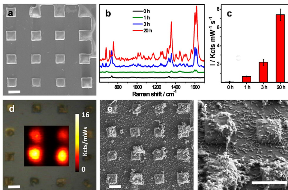
Figure 34. In situ detection and imaging of pyocyanin produced by P. aeruginosa PA14 grown on micropatterned SiO 2 -coated Au nanorod supercrystal substrates. (a) SEM images; scale bar: 5 \mu m. (b) Representative SERRS spectra measured at 0, 1, 3, and 20 h of bacteria growth. (c) Relative SERRS intensities (1600 cm -1 ), recorded at 0, 1, 3, and 20 h. (d) Optical image of the substrate and SERRS mapping of pyocyanin (1600 cm -1 ) at 20 h of growth. Scale bar: 5 \mu m. (e, f) SEM images of supercrystals colonized by P. aeruginosa (20 h) at different magnifications. Scale bar: 5 \mu m. Reproduced with permission from ref 652. Copyright 2016 Springer Nature.
